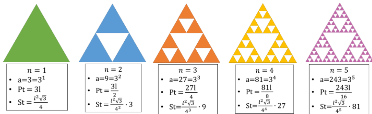
Figure 2. The first five phases of the Sierpiński triangle and the other corresponding formulas to each phase (1)
